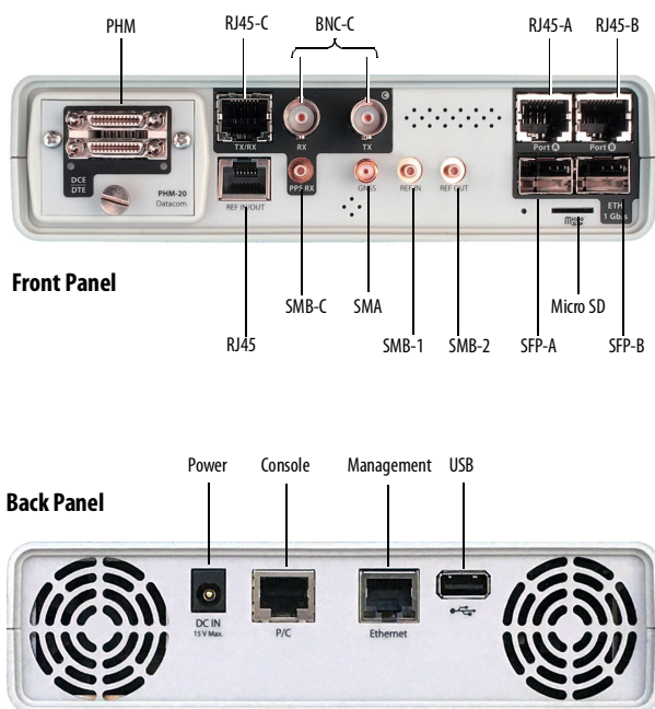
Figure 1. Ports and connectors
