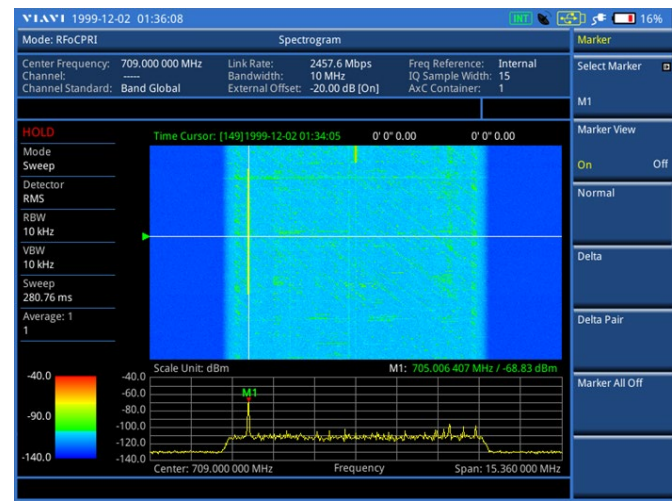
RfCPRI — Spectrogram
