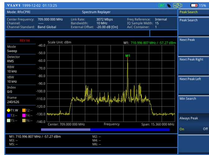
RfCPRI — Spectrum Replayer
