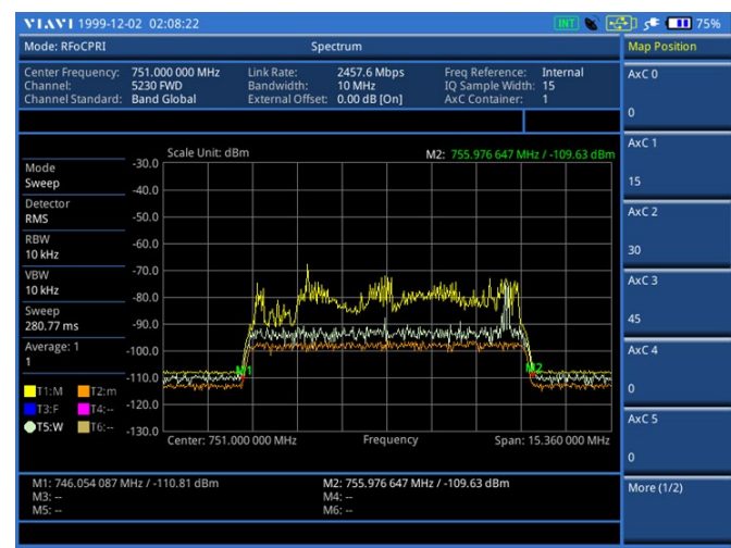
RfCPRI — Spectrum
