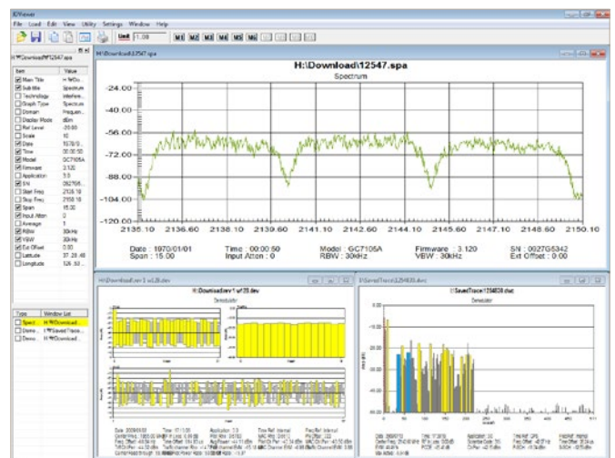
JDViewer spectrum, demodulation
