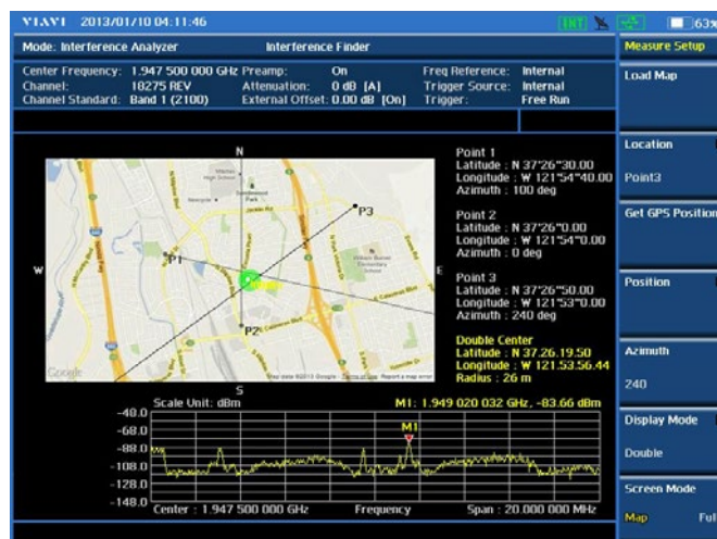
Interference analysis test — Interference Finder
