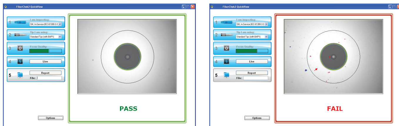
Figure 2. Example of the Proven Inspection and Analysis Software Program FiberChek2 from Viavi
