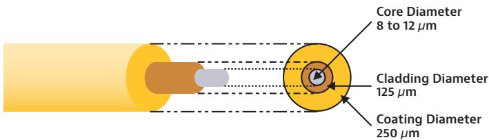
Figure 11. The composition of singlemode fiber
