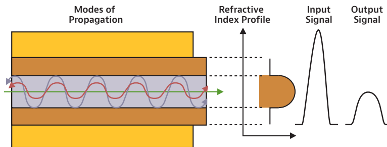
Figure 10. Light propagation through graded-index multimode fiber
