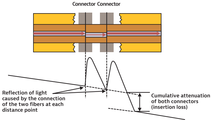
Figure 70. A reflective event at two connector junctions, which are located close together
