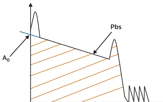
Figure 82. Total ORL measurement
