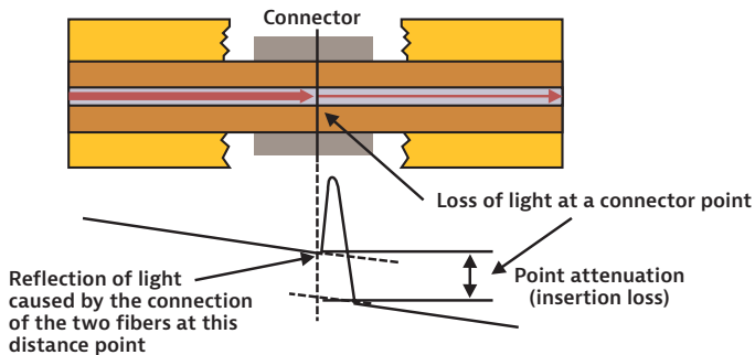
Figure 69. A reflective event at a connector junction
