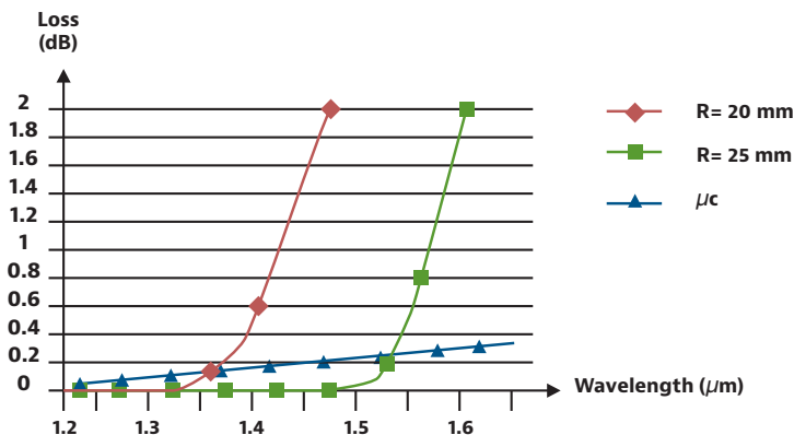
Figure 17. The effects of macro bending on a fiber
