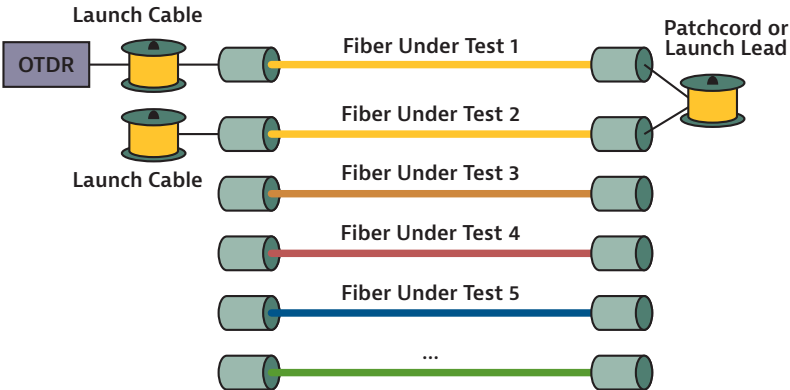
Figure 103. A loopback measurement, measuring O->E of fiber 1 and E->O of fiber 2
