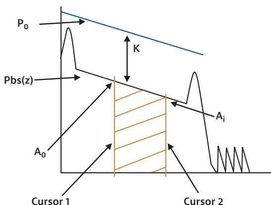
Figure 83. Section ORL measurement
