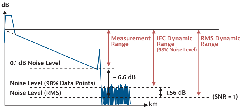
Figure 57. Different definitions of dynamic range
