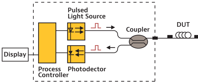
Figure 35. Setup using the OTDR method
