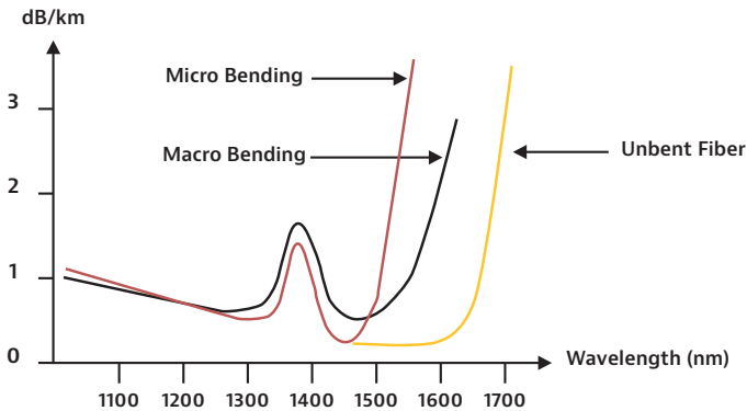
Figure 18. Typical attenuation coefficients for bent and unbent fiber
