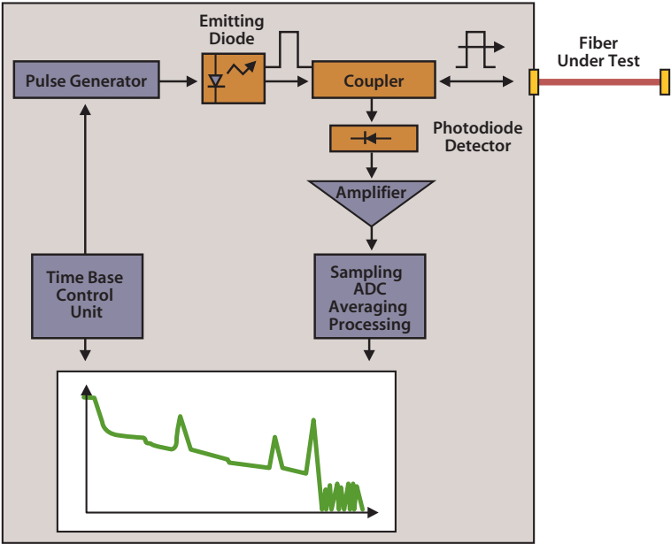
Figure 48. A schematic diagram showing OTDR technology
