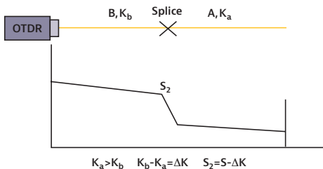
Figure 90. A negative splice from B to A
