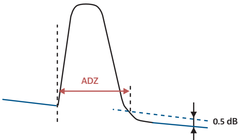
Figure 59. Measurement of the attenuation dead zone (ADZ)
