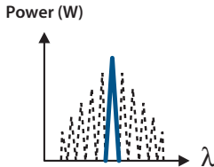
Figure 51. The emitted spectrum of a DFB laser
