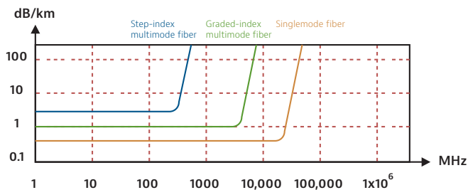
Figure 6. Typical bandwidths for different types of fiber
