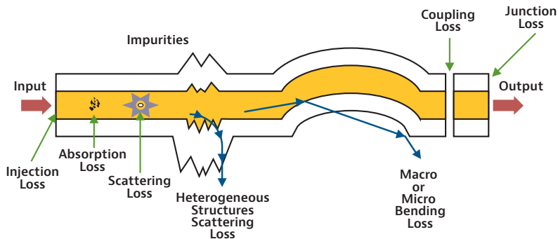
Figure 16. Link loss mechanisms
