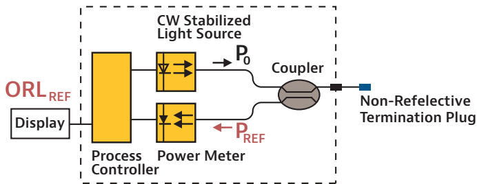
Figure 33. ORL referencing using the OCWR method
