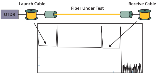
Figure 99. Acceptance testing using launch and receive cables
