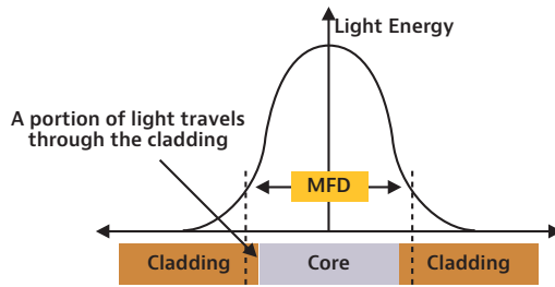
Figure 12. The mode field diameter (MFD) of singlemode fiber
