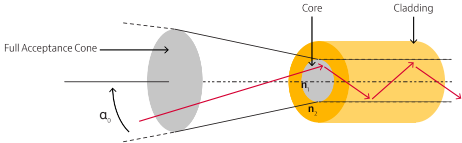
Figure 2. The injection of light into a fiber
