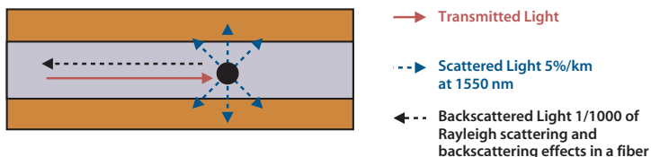
Figure 45. Rayleigh scattering and backscattering effects in a fiber
