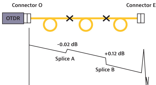
Figure 95. OTDR measurement from connector O to connector E (O->E)
