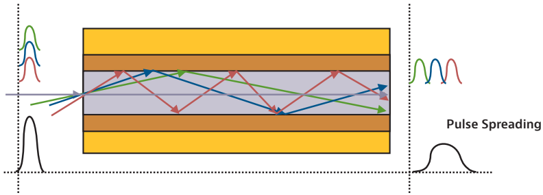
Figure 20. Modal dispersion in step-index multimode fiber
