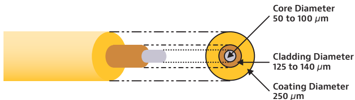
Figure 8. The composition of multimode fiber
