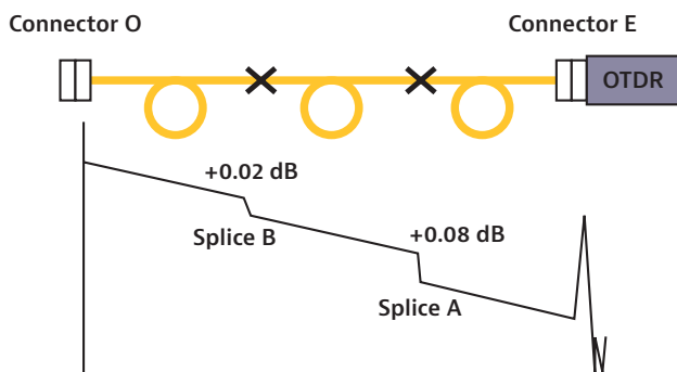
Figure 96. OTDR measurement from connector E to connector O (E->O)
