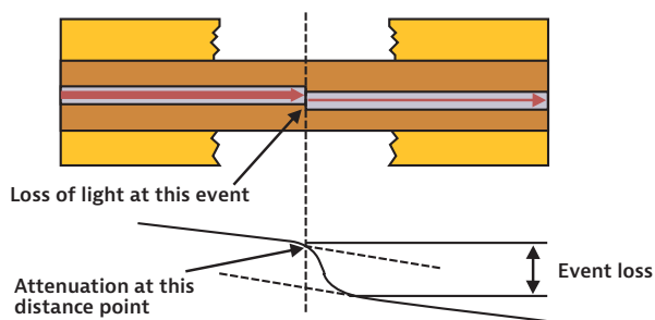
Figure 72. A non-reflective event
