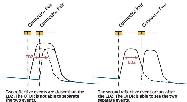
Figure 63. Event dead zone and connector discrimination by the OTDR
