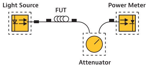
Figure 31. The use of an optical attenuator in optical testing
