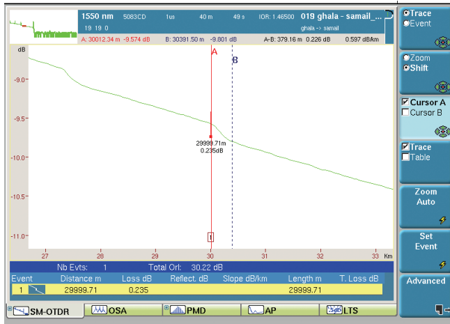
Figure 77. The least squares approximation method
