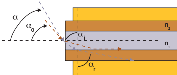
Figure 3. Refraction of light
