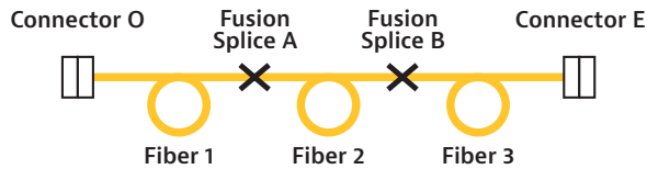
Figure 91. The span architecture
