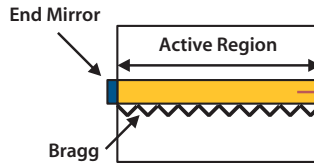
Figure 52. A schematic diagram of a DFB laser
