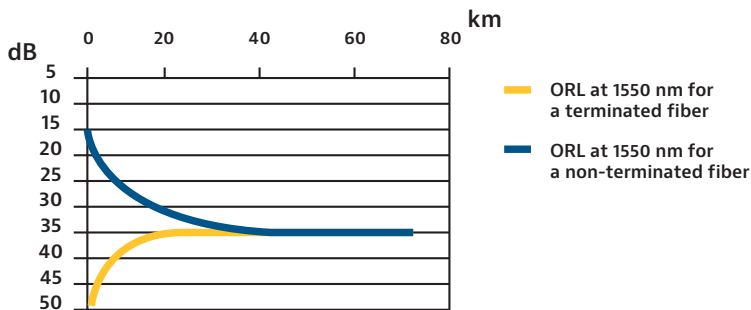
Figure 23. ORL as a function of distance at 1550 nm for terminated and non-terminated fiber
