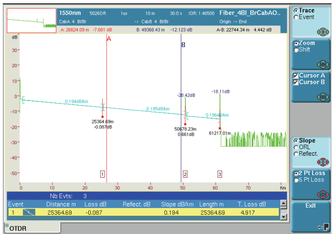
Figure 75. Manual measurement using cursors A and B
