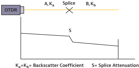
Figure 88. A normal splice
