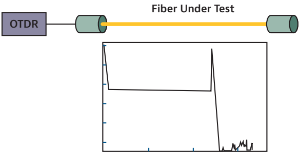
Figure 98. Acceptance testing without the use of launch and receive cables
