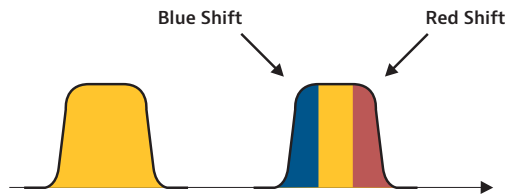
Figure 25. Self phase modulation of a signal on a fiber
