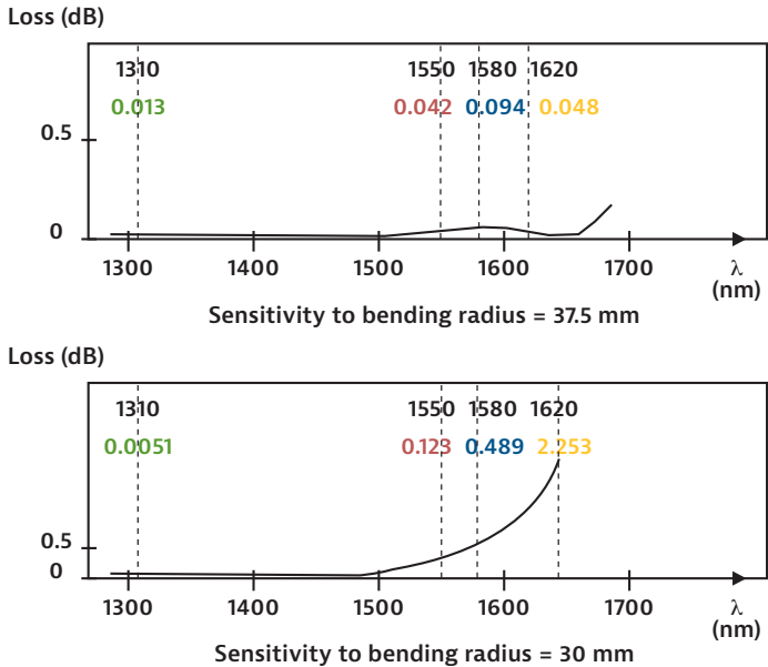
Figure 64. The effects of bending on a fiber
