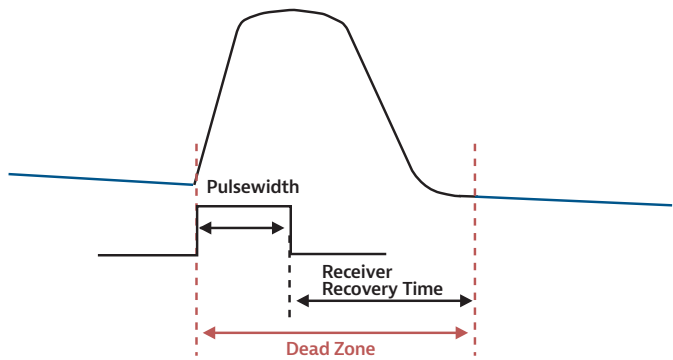
Figure 58. The OTDR dead zone
