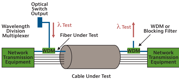
Figure 44. In-service monitoring of a link
