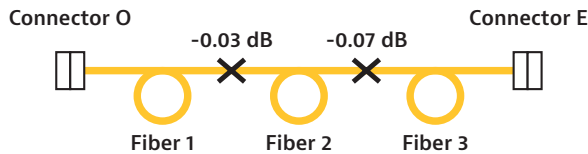
Figure 94. Actual fusion splice loss
