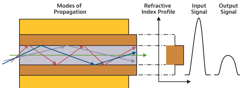
Figure 9. Light propagation through step-index multimode fiber
