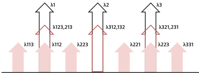
Figure 24. Four wave mixing of a signal on a fiber
