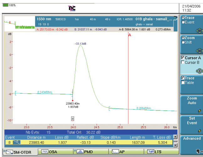
Figure 80. Reflectance measurement
