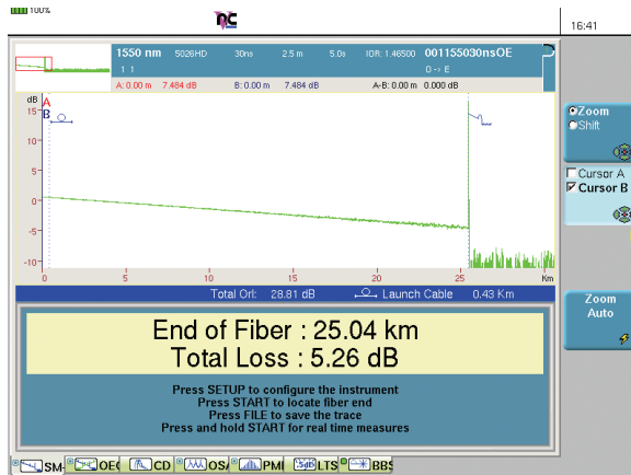
Figure 101. Fault location using an OTDR
