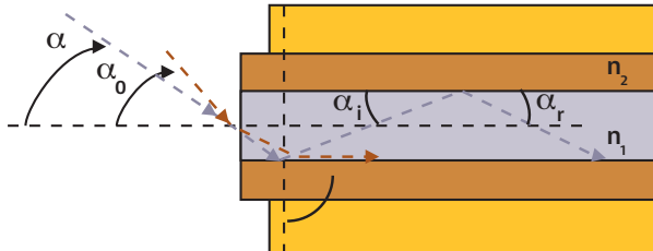
Figure 4. Reflection of light
