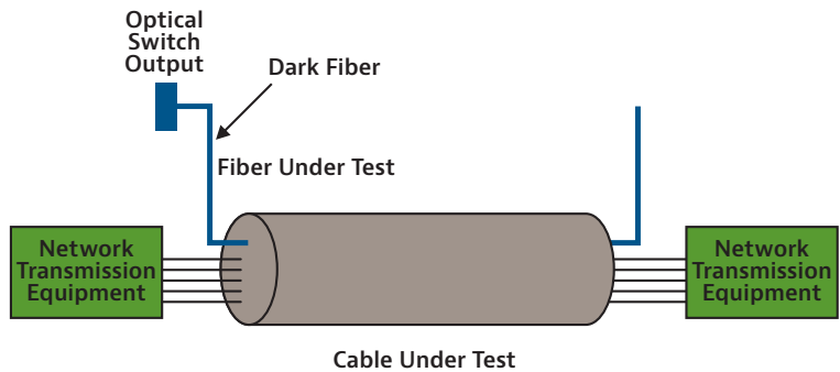
Figure 43. Out-of-service monitoring of a link
