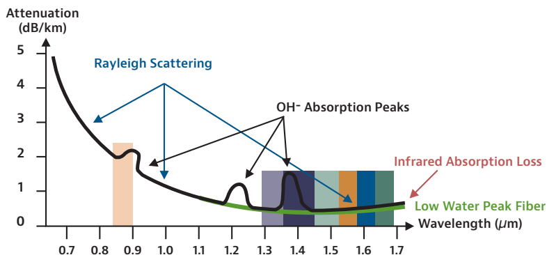
Figure 15. Fiber attenuation as a function of wavelength
