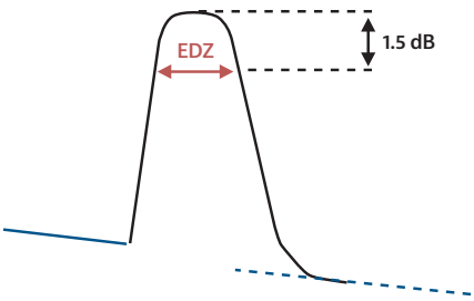
Figure 61. The event dead zone (EDZ) of a reflective event
