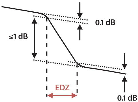
Figure 62. The event dead zone (EDZ) of a non-reflective event
