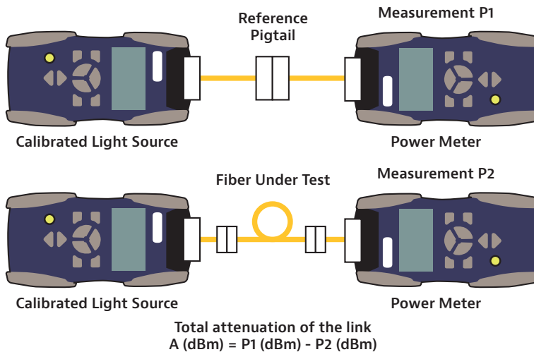
Figure 28. The insertion loss method uses two steps to measure the attenuation along a fiber link
