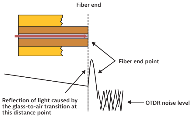
Figure 71. A reflective event at a fiber end
