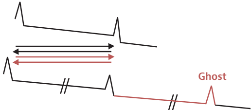
Figure 84. Ghosts on an OTDR trace
