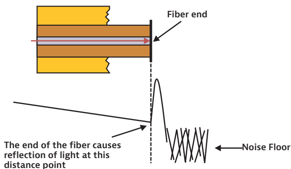
Figure 100. Break or fiber end location
