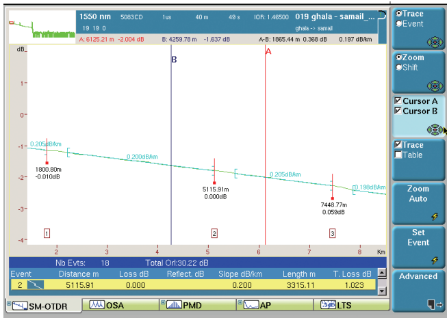
Figure 74. Semi- automatic event detection using the VIAVI T-BERD/MTS platforms
