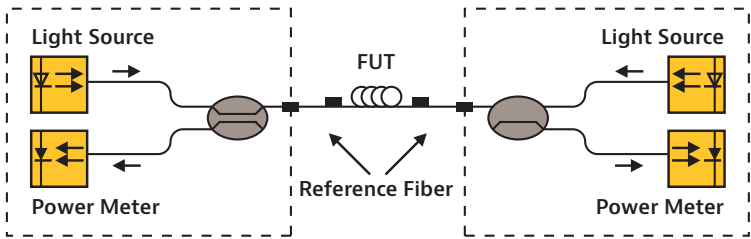
Figure 29. Insertion loss measurement with two bi-directional loss test sets
