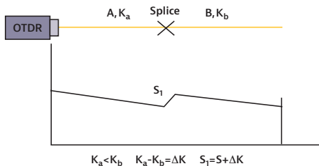
Figure 89. A positive splice A to B
