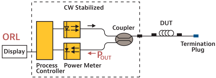
Figure 34. ORL measurement using the OCWR method
