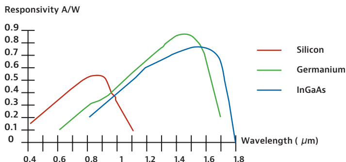
Responsivity of the three typical detector types
