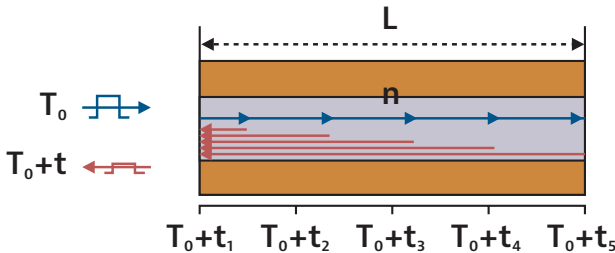
Figure 55. The OTDR pulse generation principle
