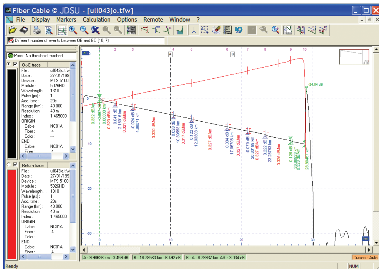
Figure 105. Bidirectional analysis using VIAVI FiberCable software
