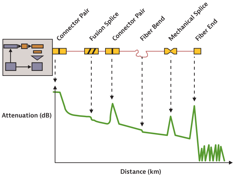
Figure 56. A typical OTDR trace
