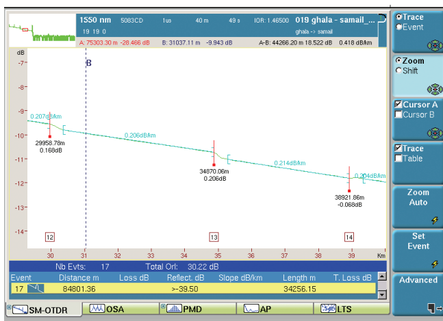
Figure 79. 5-Point Measurement Method
