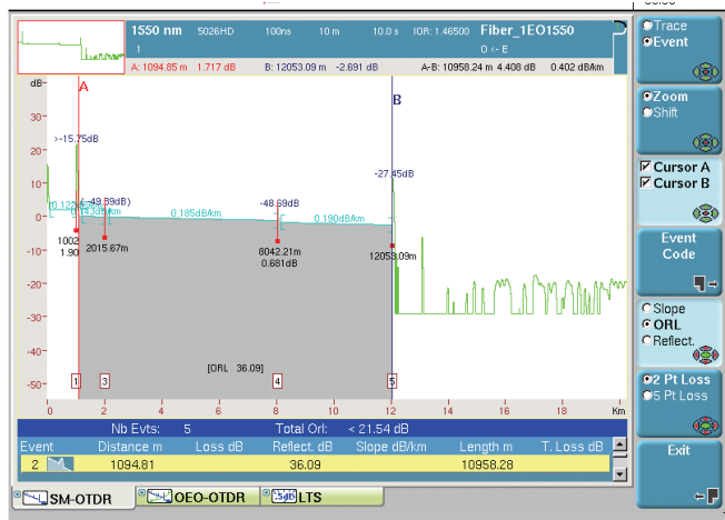
Figure 81. ORL measurement of a fiber link
