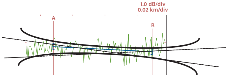
Figure 76. Using the 2-point measurement method between cursors A and B
