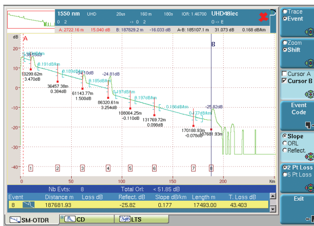
Figure 73. Automatic event detection using the VIAVI T-BERD/MTS platforms
