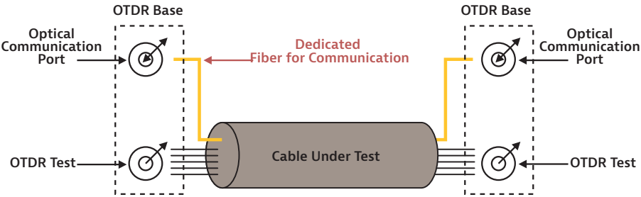
Figure 102. Automatic bidirectional OTDR measurement configuration
