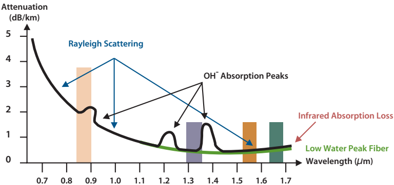
Figure 46. Fiber attenuation as a function of wavelength
