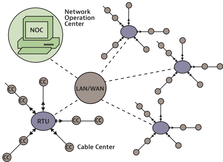
Figure 42. A remote monitoring system
