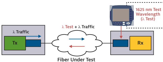
Figure 66. In-service testing at 1625 nm using the contra-propagation method
