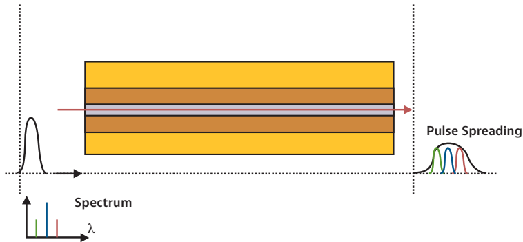
Figure 21. Chromatic dispersion caused by different wavelengths in a light source
