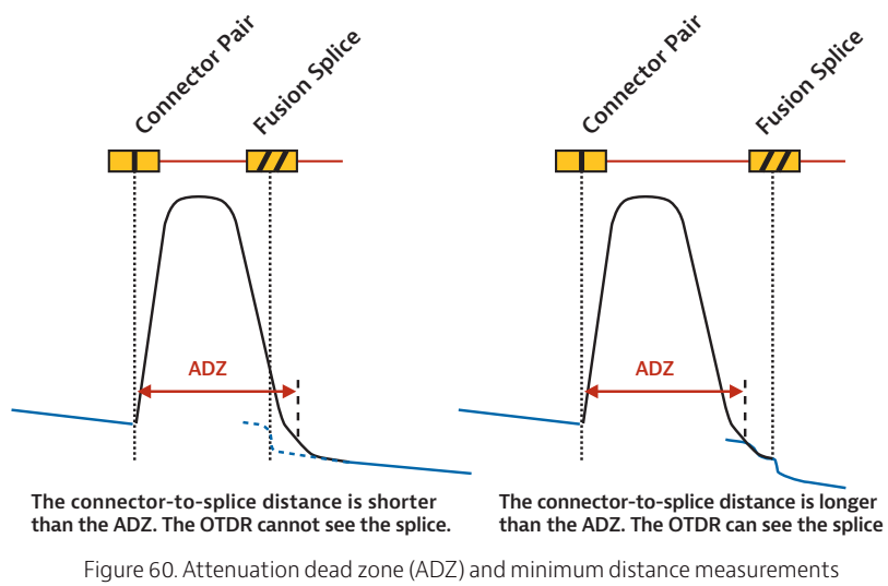
Figure 60. Attenuation dead zone (ADZ) and minimum distance measurements
