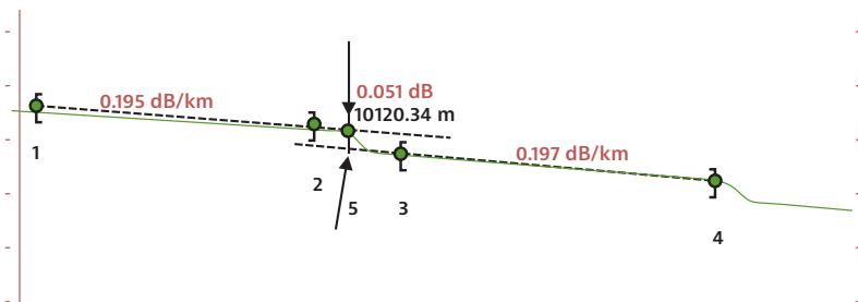
Figure 78. Using the 5-point measurement method
