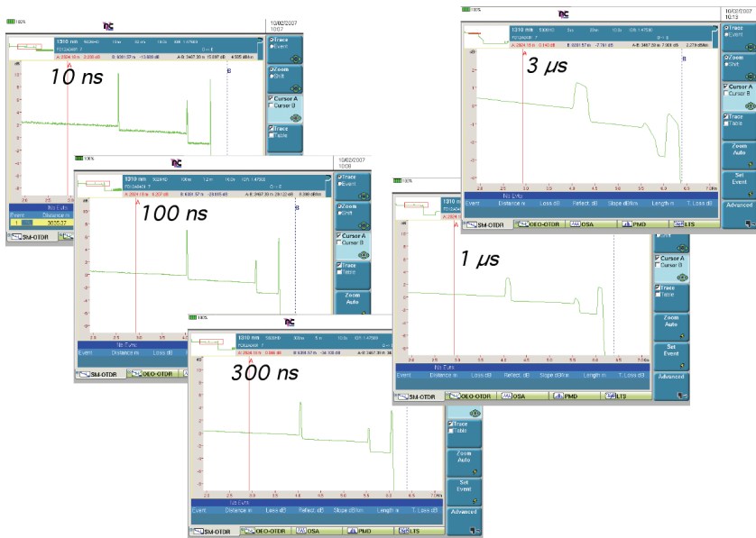
Figure 67. Fiber measurement using different pulsewidths
