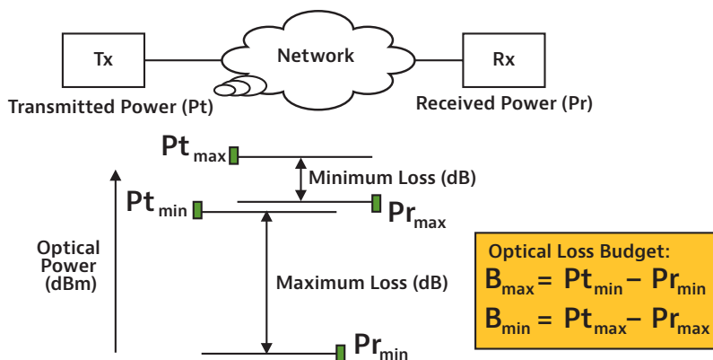
Figure 32. Calculating the optical loss budget
